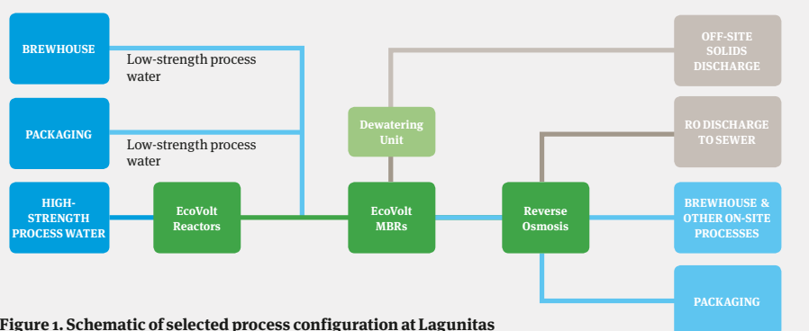
Figure 1. Schematic of selected process configuration at Lagunitas Brewing Company. Provided by Cambrian Innovation
